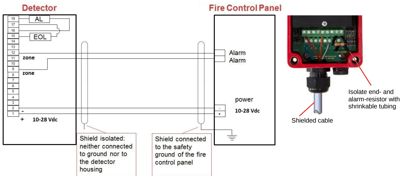
Connection diagram
